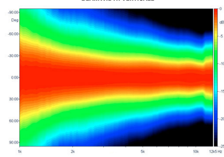
BEAMWIDTH VERTICALE
