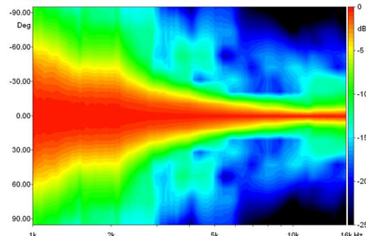
BEAMWIDTH VERTICALE
