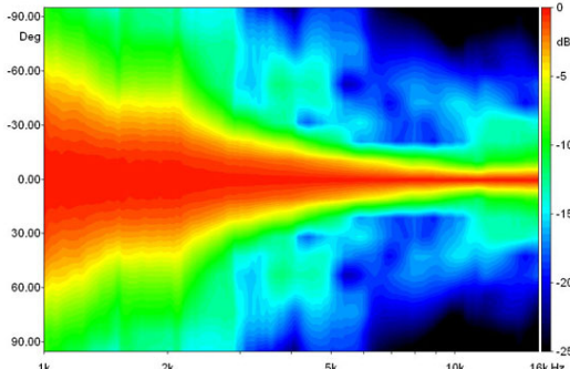
BEAMWIDTH VERTICALE
