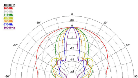
VERTICAL POLAR PATTERN
