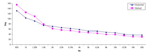
VERTICAL BEAMWIDTH
