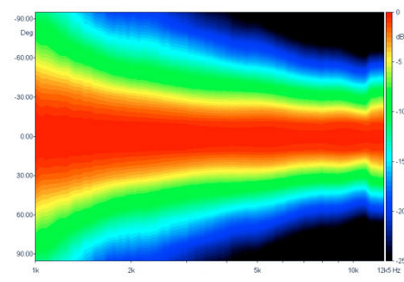
BEAMWIDTH VERTICALE
