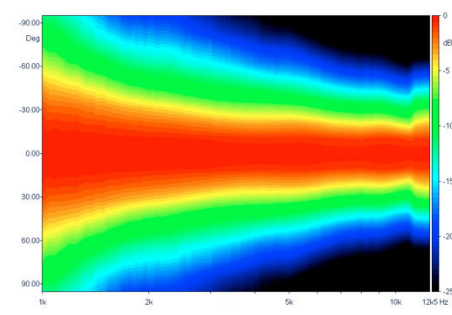
BEAMWIDTH VERTICALE
